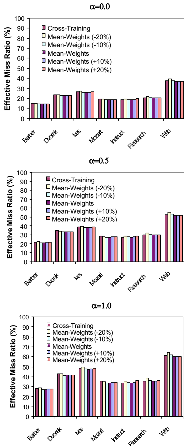
Figure 5: Effect of Heuristic Weight Computation Method on Performance.
