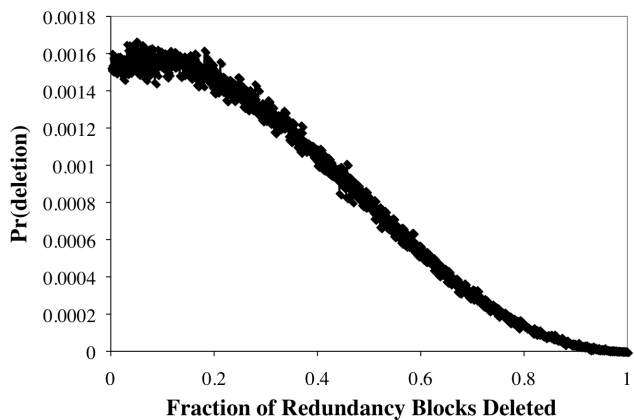
Figure 2: Identify the best attack strategy by varying where blocks are deleted.
