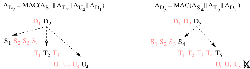
Figure 2: Updating directory version authenticators when file U is deleted.
